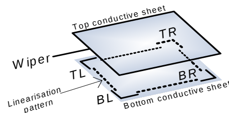
Figure 11. 5-wire touchscreen
