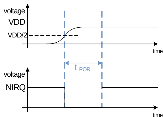
Figure 13. Power-up, NIRQ
