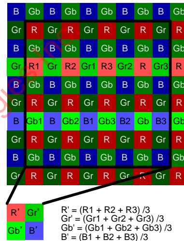
Vertical 2/8 Subsampling Binning Horizontal 3 Binning Binning Image
