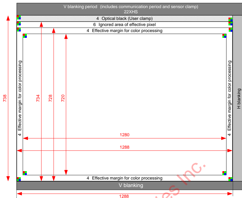
Readout Pixel Image Diagram (1280 x 720)
