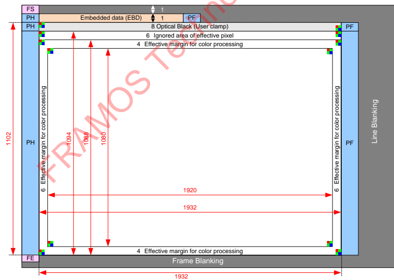
Readout Pixel Image Diagram (1920 x 1080)
