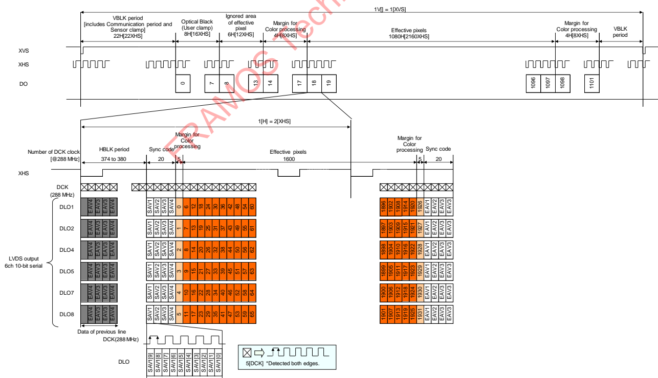
Readout Drive Timing
