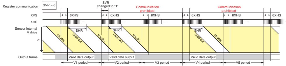
Example of SVR operation
