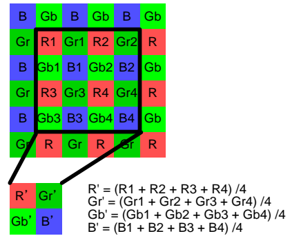
Horizontal/Vertical 2/2-line Binning (no weighted binning) Binning Image
