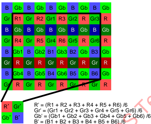
Vertical 2/3 Subsampling Binning Horizontal 3 Binning Binning Image
