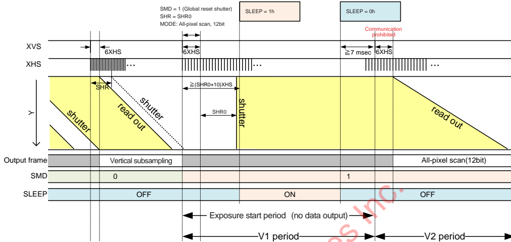
Low Power Consumption Drive in Exposure of Global Reset Shutter Operation Sequence (Sub-LVDS)
