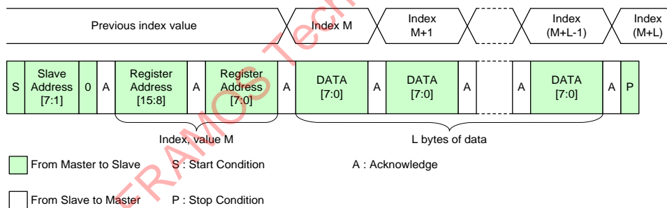
Sequential Write Starting from Random Location
