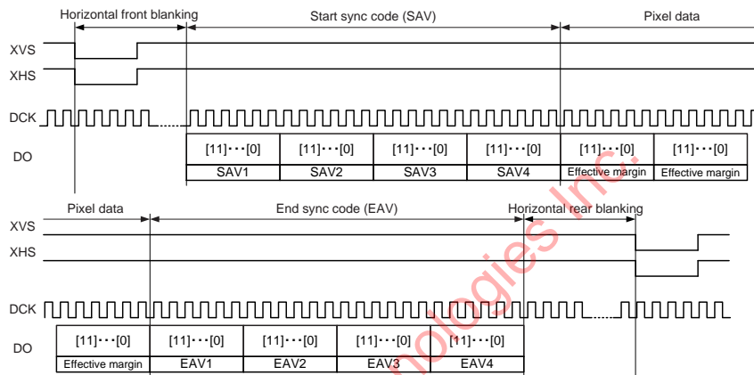
Sync Signal and Data Output Timing
