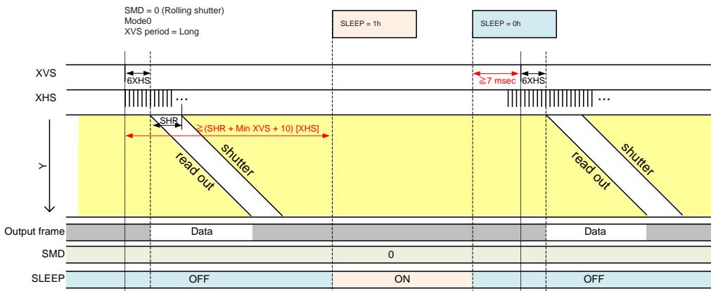
Low Power Consumption Drive in Integrational Time When Using Rolling Shutter Operation (Sub-LVDS)
