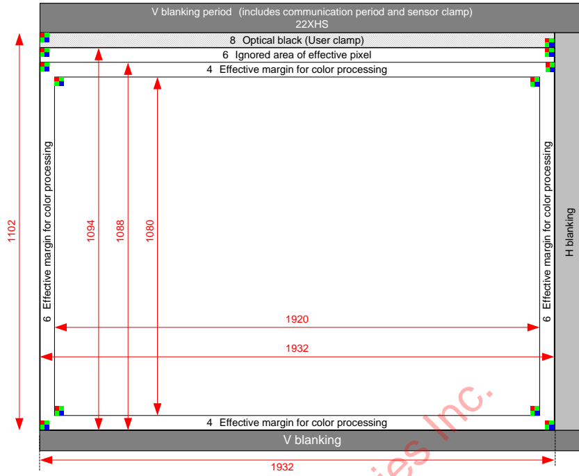
Readout Pixel Image Diagram (1920 x 1080)
