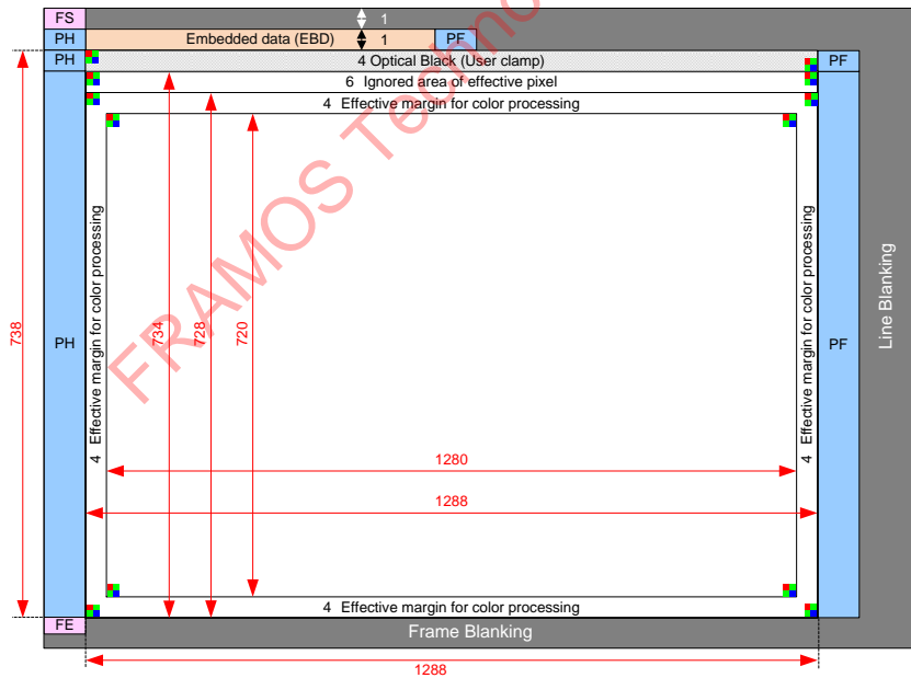
Readout Pixel Image Diagram (1280 × 720)
