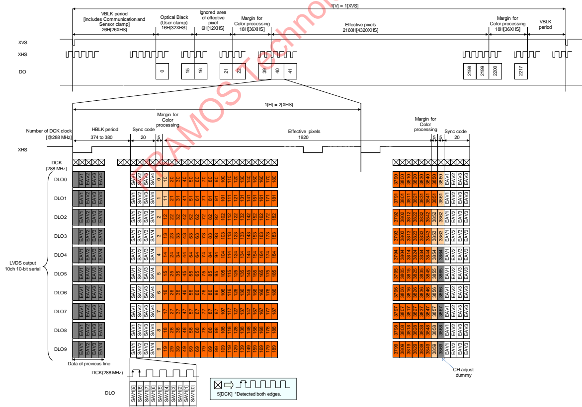
Readout Drive Timing
