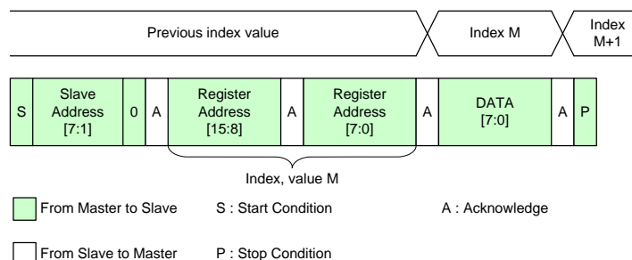
Single Write to Random Location
