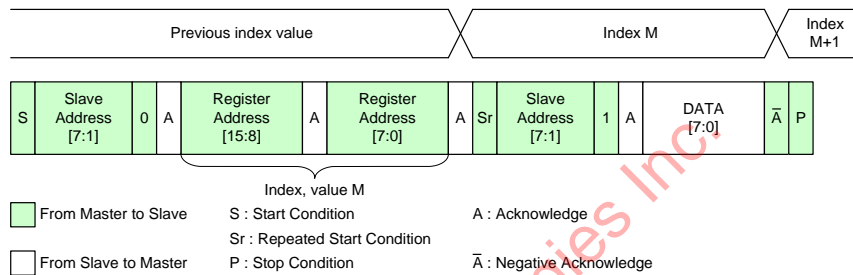
Single Read from Random Location
