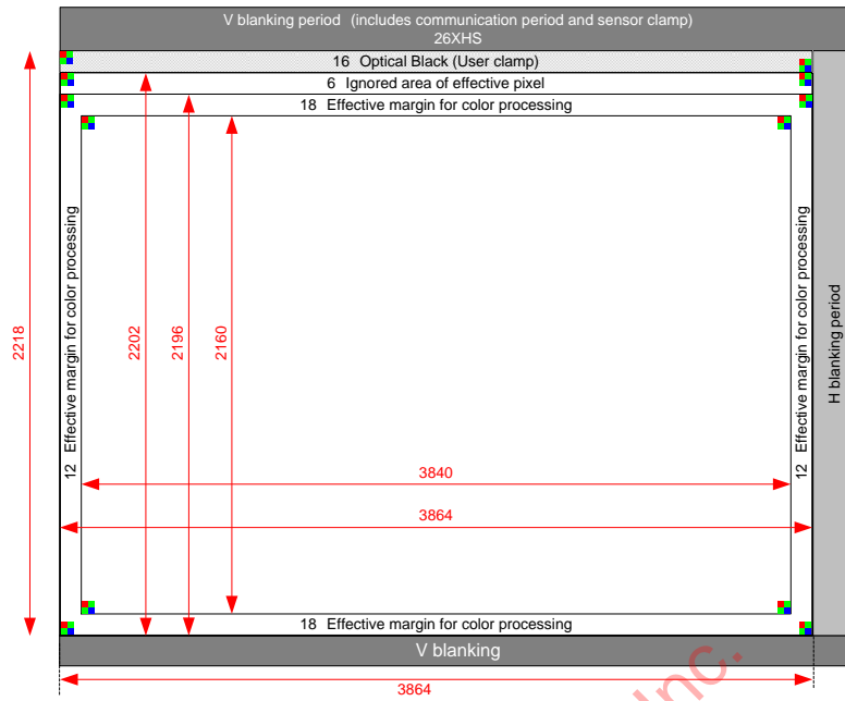
Readout Pixel Image Diagram (3840 x 2160)
